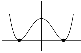
Figure 5.1: The graph of the double-well potential.
